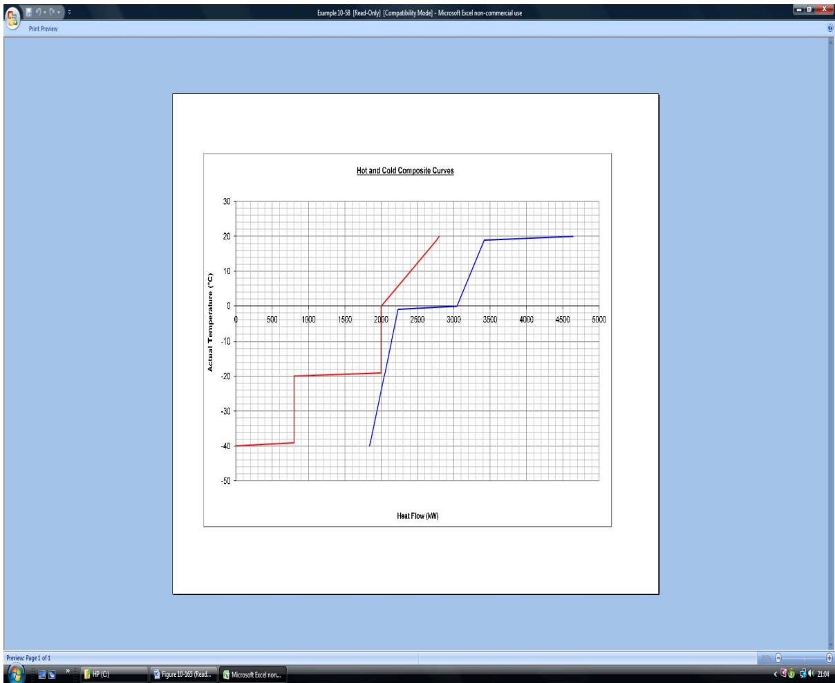
Figure 10-165. A screen-shot of hot and cold composite curves vs. heat flow for Example 10-58.
